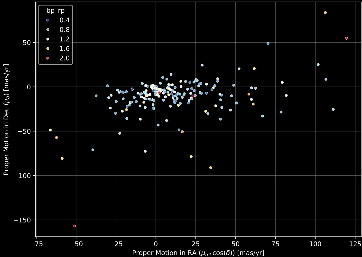
APOGEE DR17 Field: [101-45_MGA] Proper Motion Diagram (n= 198)
