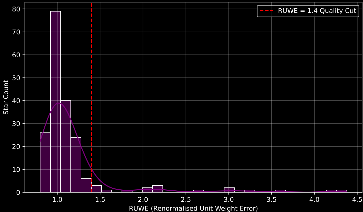
GAPOGEE DR17 Field [101-45_MGA] RUWE Distribution (n= 192)
