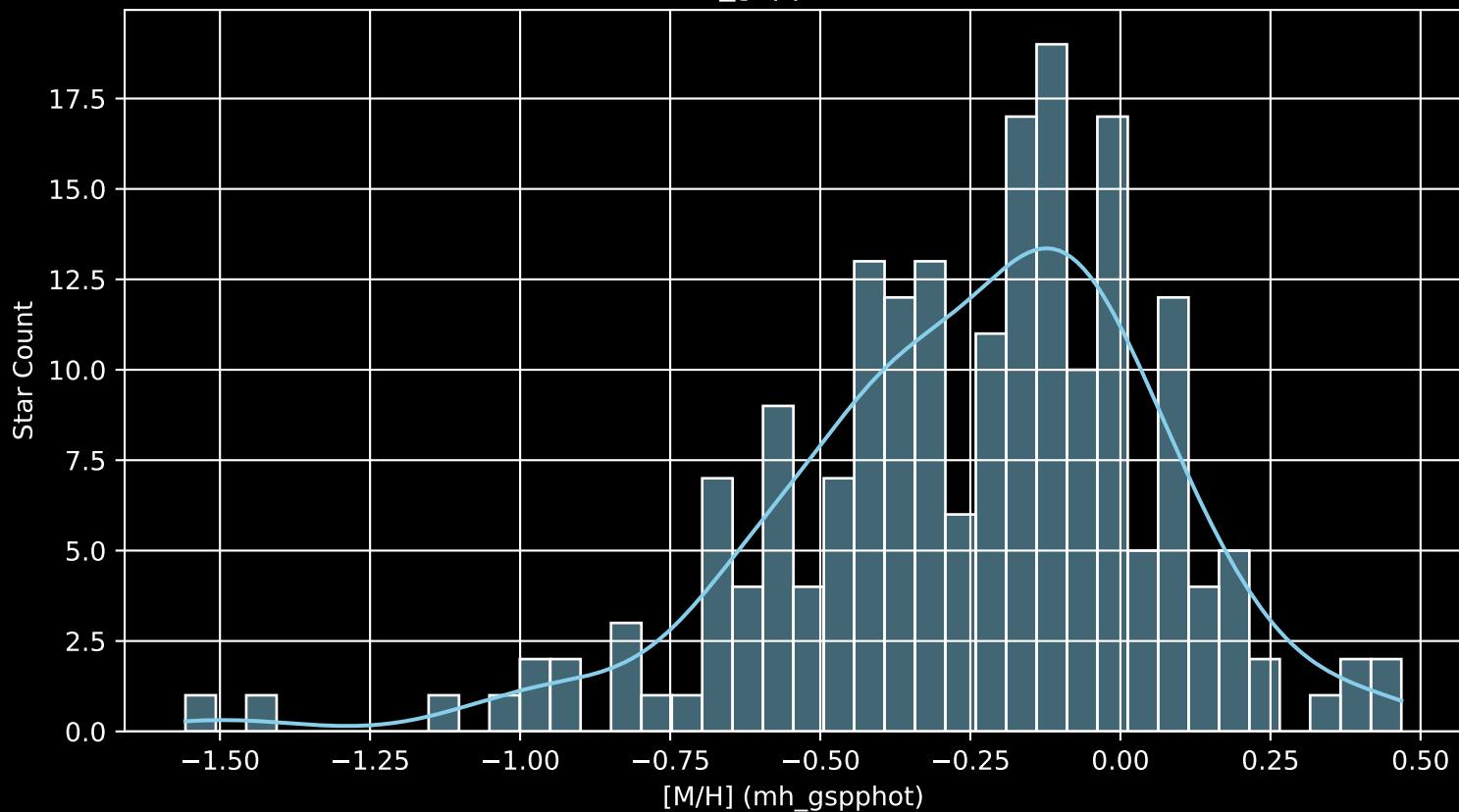
APOGEE DR17 Field: [101-45_MGA [M/H] (mh_gspphot) (n= 195)
