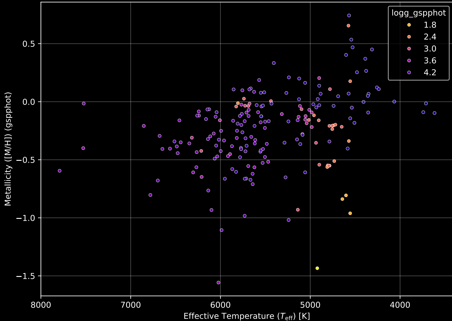
APOGEE DR17 Field: [101-45_MGA] Stellar Population Parameters (n= 198)
