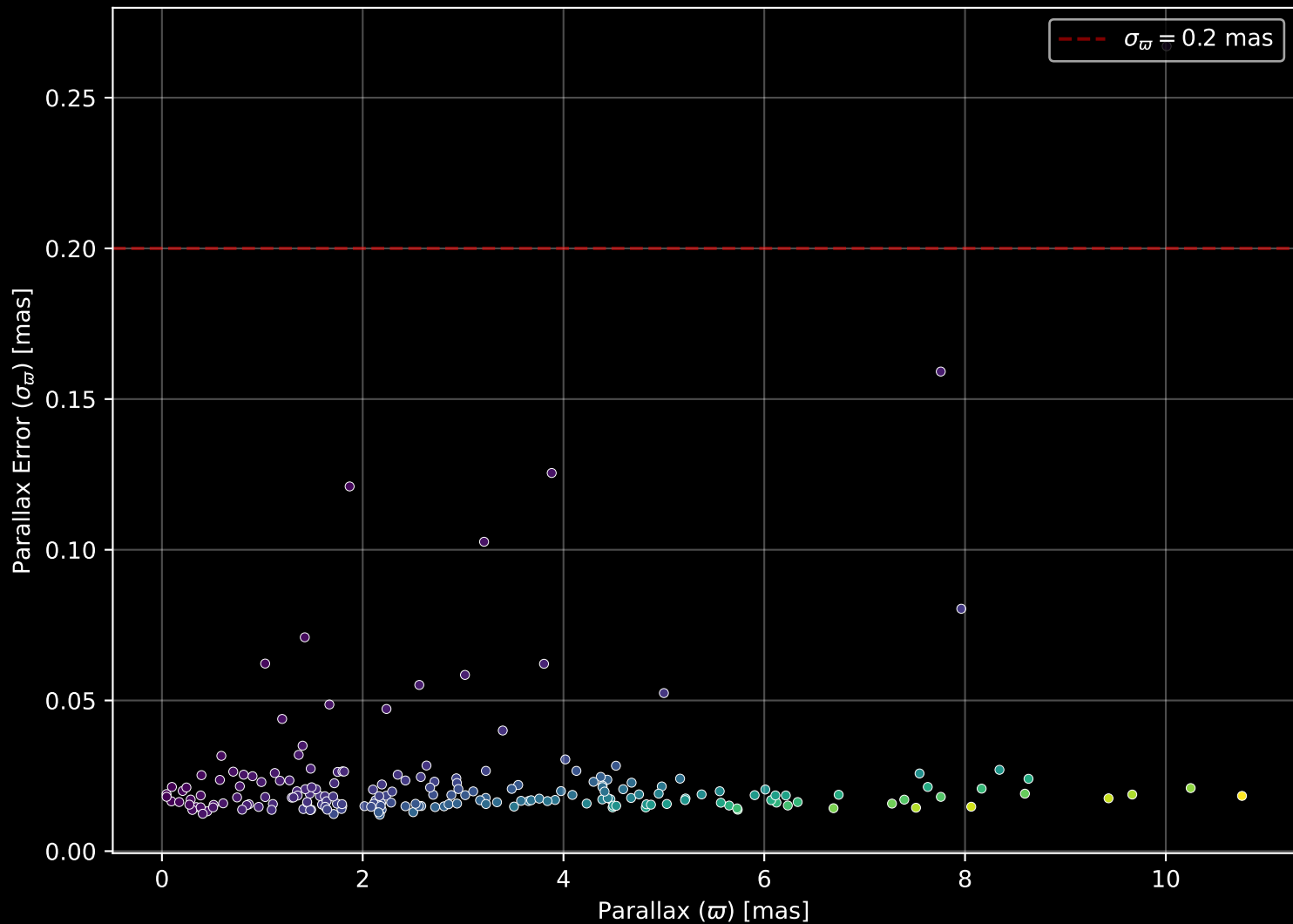
APOGEE DR17 Field: [101-45_MGA] Parallax Quality (n= 198)
